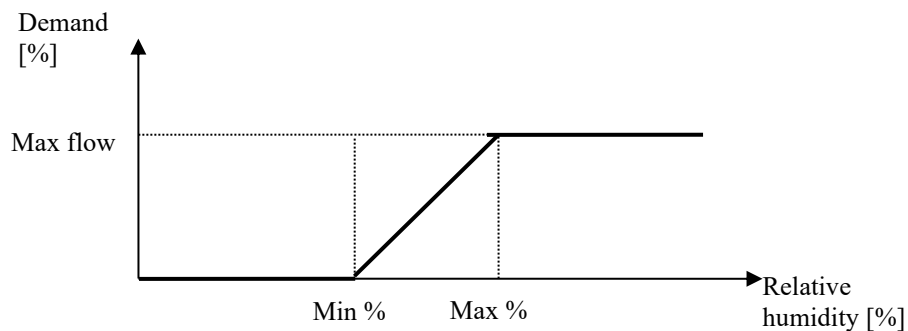
Figure 19: Dehumidification controller curve
