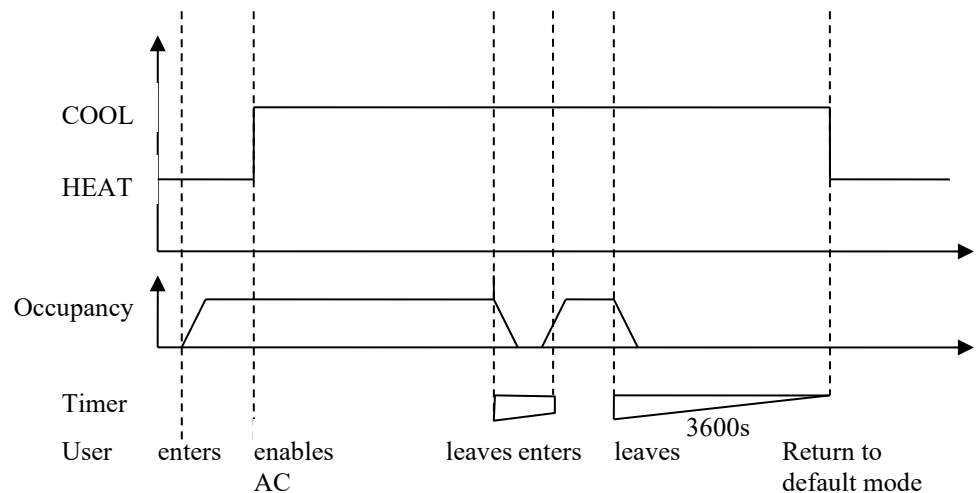
Figure 11: Example timing behavior of HVAC default mode (HEAT) and HVAC default delay (3600s).
