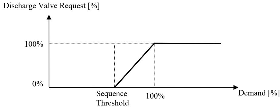
Figure 23: Inverse sequencing of the valve control signal
