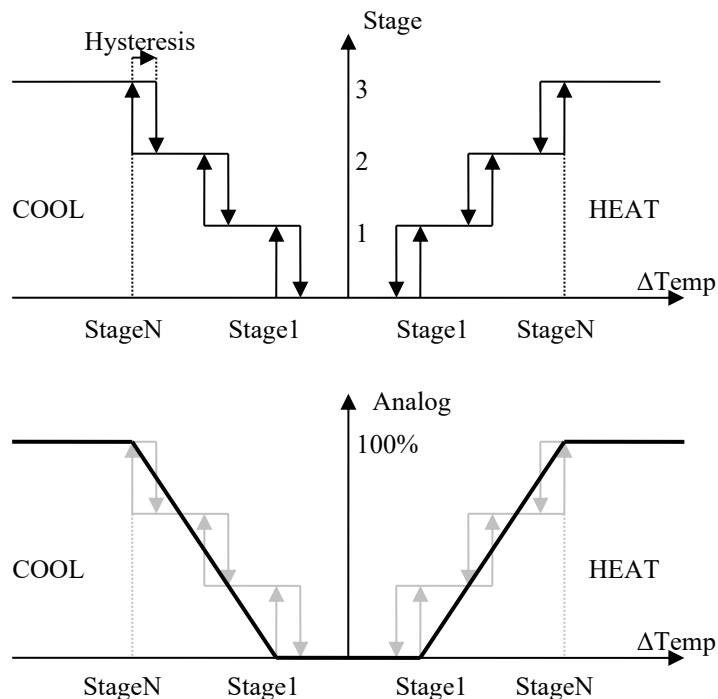
Figure 27: Fancoil sequence
