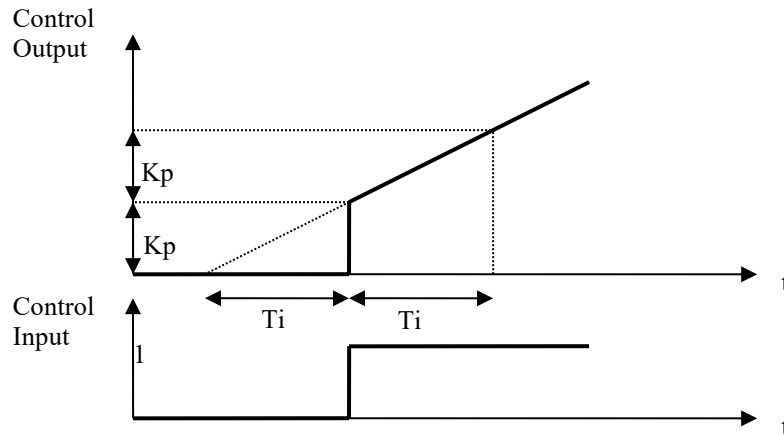
Figure 17: PI Controller step response
