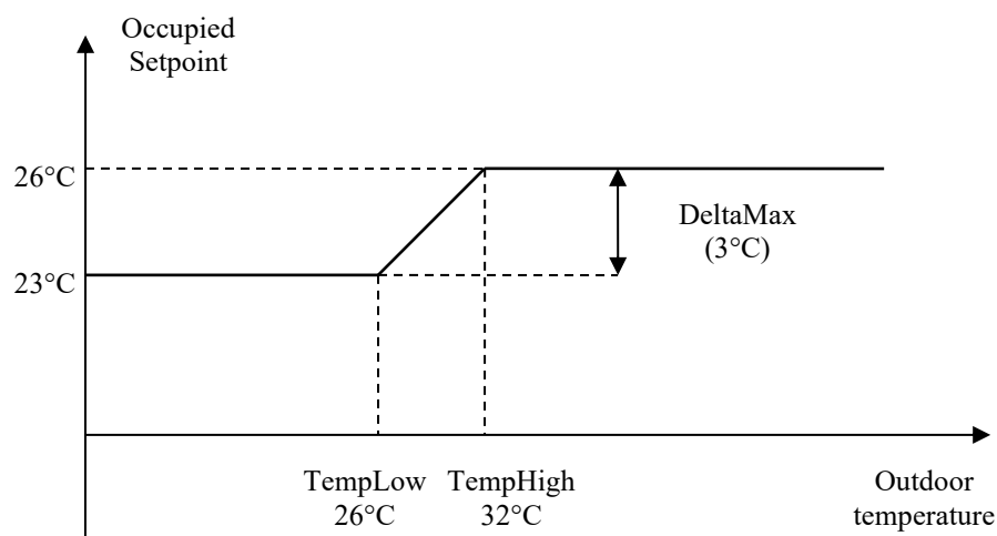
Figure 15: Summer Compensation.
