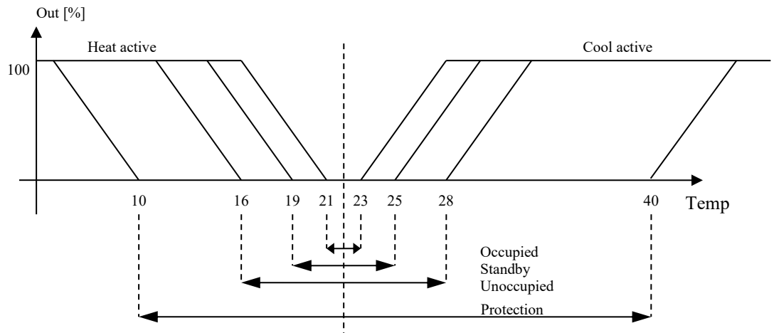
Figure 12: Setpoints and control output.
