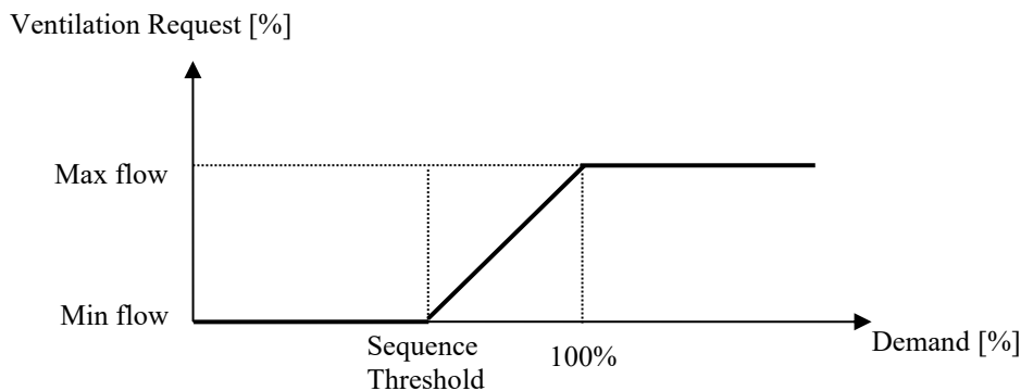
Figure 20: Sequencing of the ventilation request
