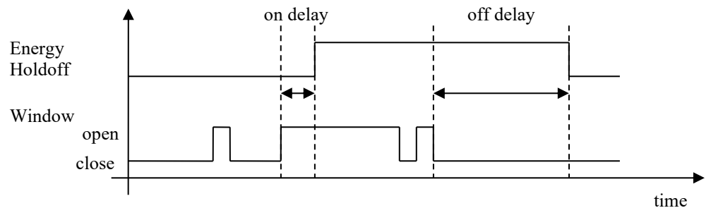
Figure 14: Energy holdoff timing.
