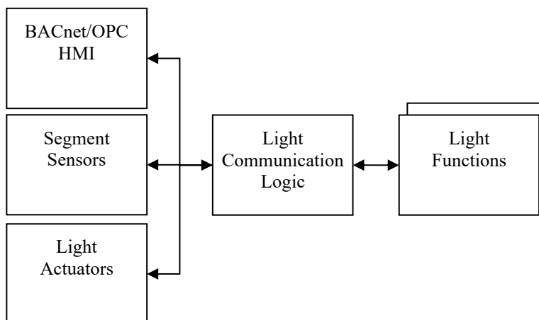
Figure 32: Light controller
