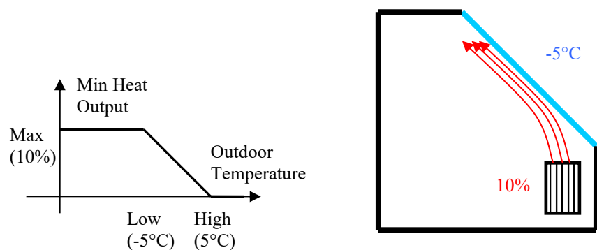
Figure 16: Minimum heating function
