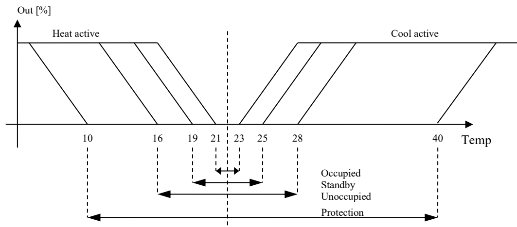
Figure 12 shows the default setpoints and the control output with varying temperature (shown without the time-dependent integral component).
