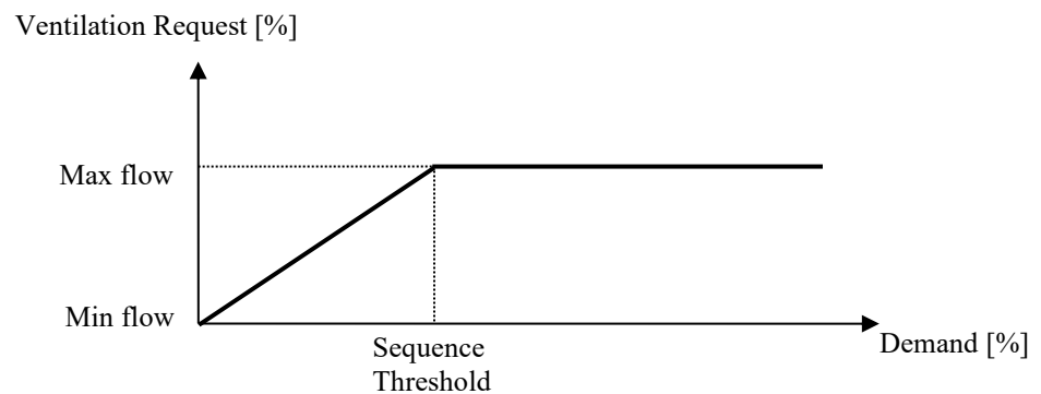
Figure 22: Inverse sequencing of the ventilation demand
