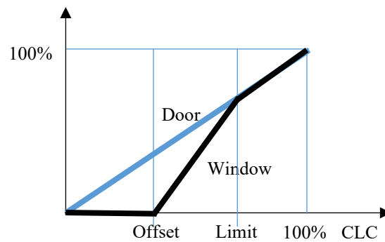
Figure 34: Window band parameters
