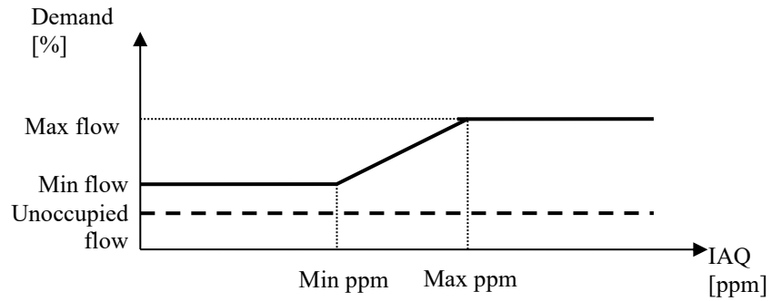
Figure 18: IAQ controller curve
