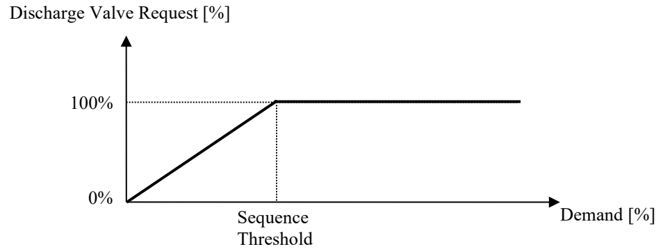
Figure 21: Sequencing of the discharge valve request
