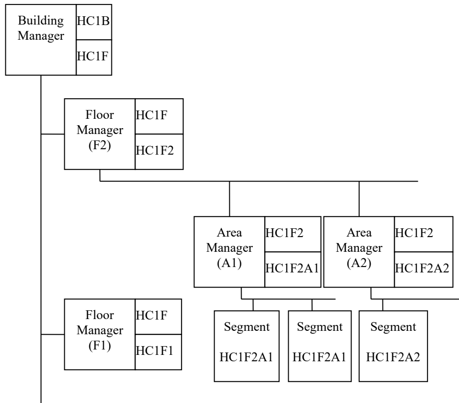
Figure 30: Heating Circuit IDs for heating circuit 1 (HC1).
