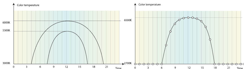
Figure 35: HCL profiles “Elevation” based on different values for summer/winter (left) and “Curve_Daily” with reference points for each full hour (right)
