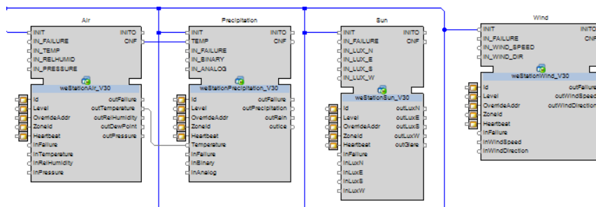
Figure 7: Standard weather station.
