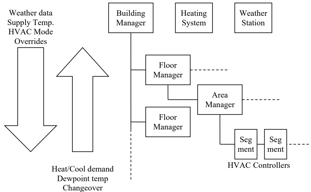
Figure 10: L-ROC HVAC Components
