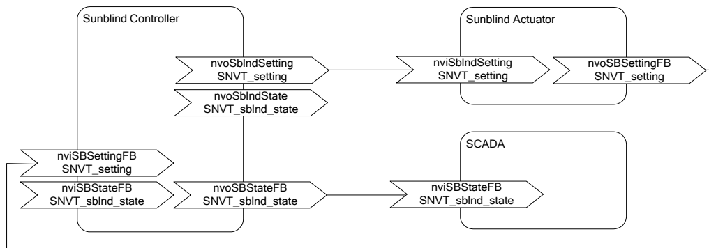
Figure 124: Controlling a Sunblind Actuator via SNVT_setting
