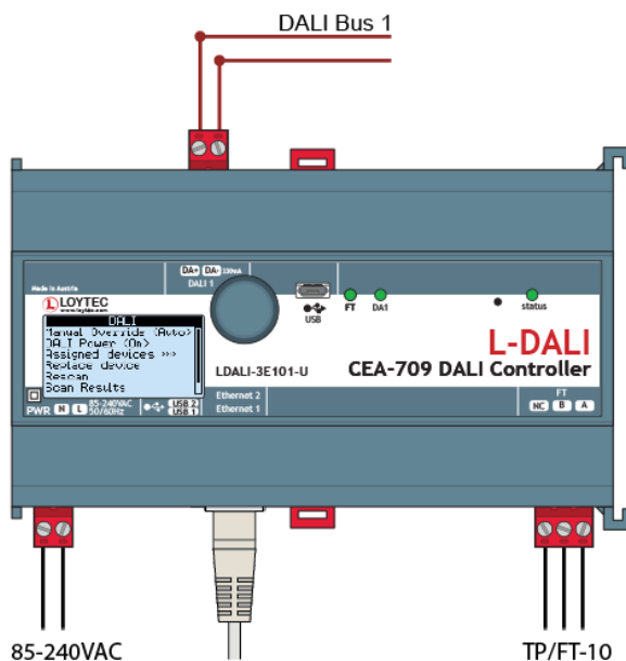
Figure 66: Basic Hardware Installation with integrated DALI bus power.
