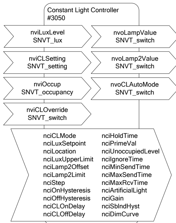
Figure 112: Constant Light Controller Object
