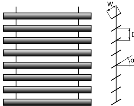
Figure 122: Sunblind Geometry
