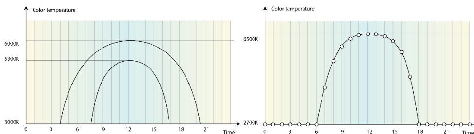
Figure 119: HCL Profile "elevation" based with different Tc max values for summer and winter (left) and "curve daily" with hourly support values (right)
