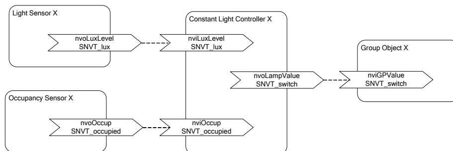
Figure 113: Default Connections to other LONMARK Objects
