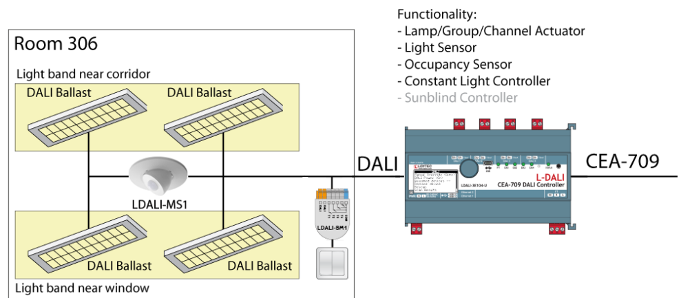
Figure 64: Quick-Start Example Project.
