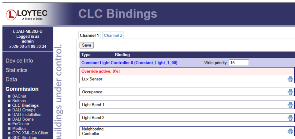
Figure 147: CLC binding with an active manual override.
