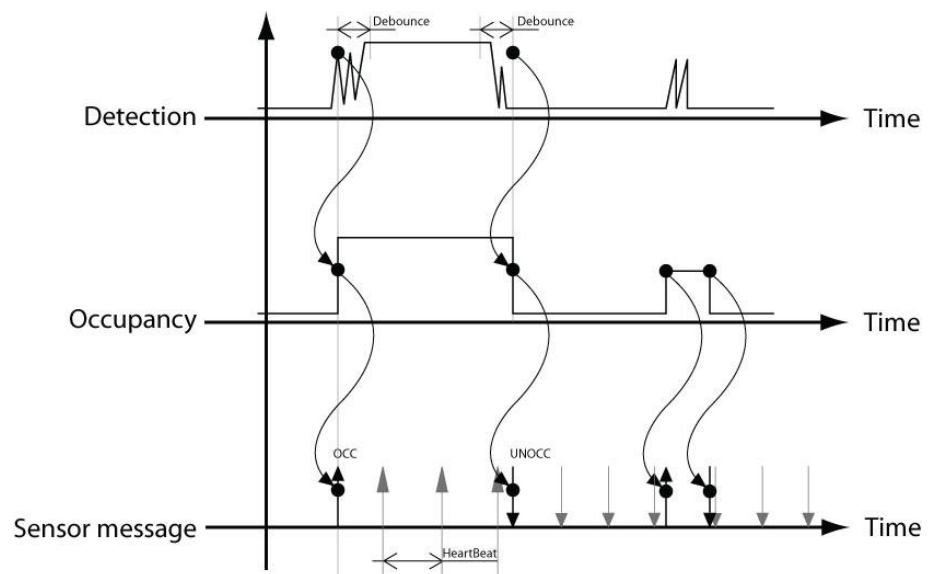
Figure 111: Timing of occupancy detection.
