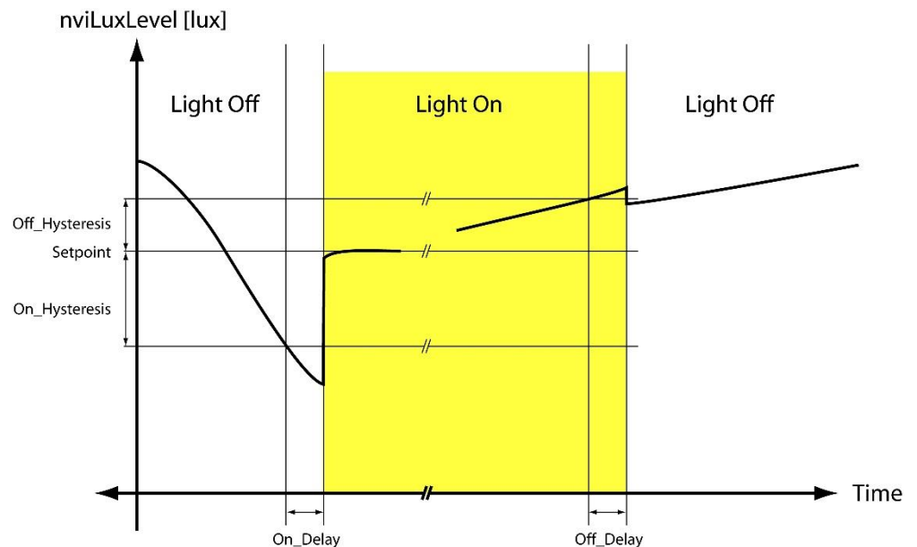
Figure 140: Constant Light Controller Timing.
