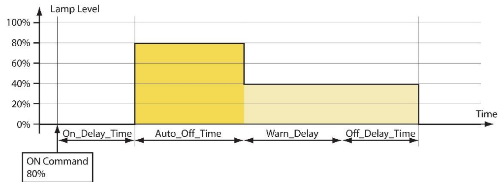
Figure 132: Timing Parameters with Auto_Off_Time and Warn_Delay .
