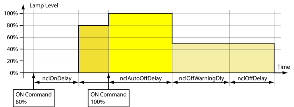
Figure 106: Timing Parameters ( nciAutoOffRestart=ST_ON )
