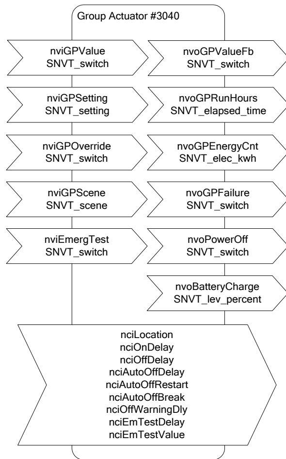
Figure 102: Group Actuator Object
