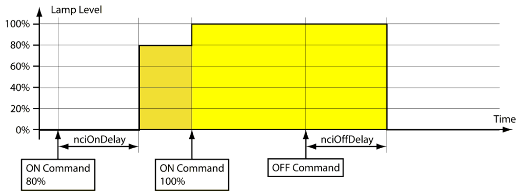
Figure 104: Timing Parameters
