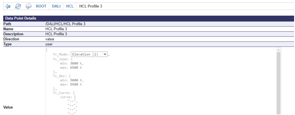
Figure 120: HCL Profile 3 - elevation based with different Tc max values for summer and winter
