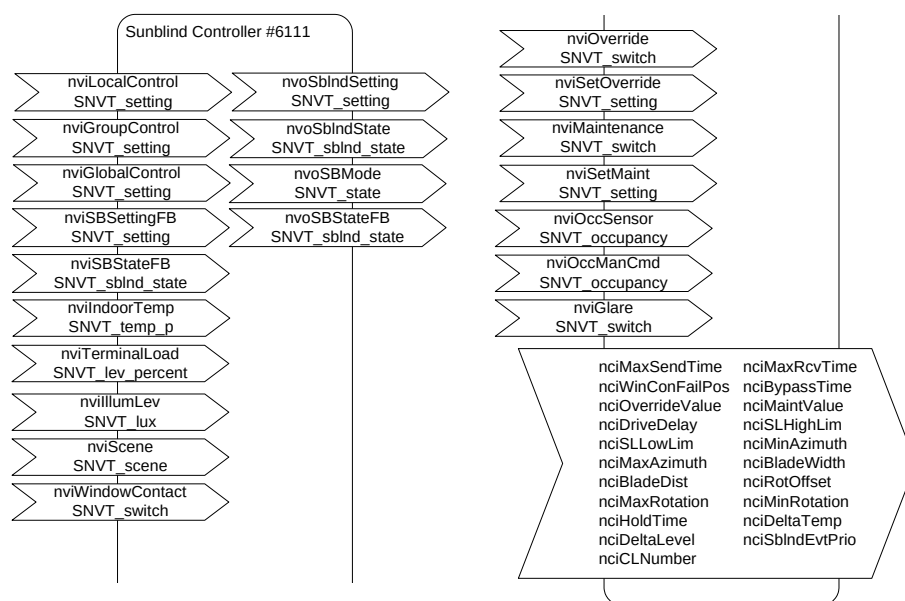
Figure 121: Sunblind Controller Object
