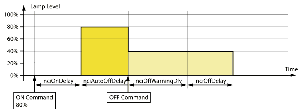
Figure 107: Timing Parameters ( nciAutoOffBreak=ST_ON )
