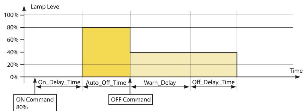
Figure 134: Timing Parameters (break enabled).
