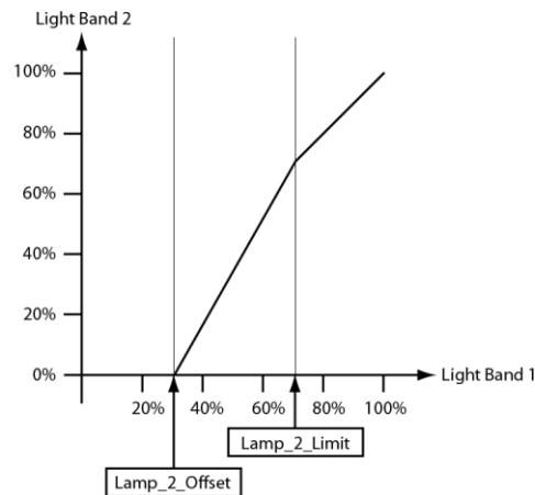
Figure 139: Secondary Light Band
