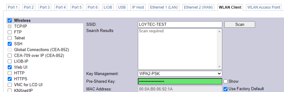
Figure 21: New WLAN configuration tabs
