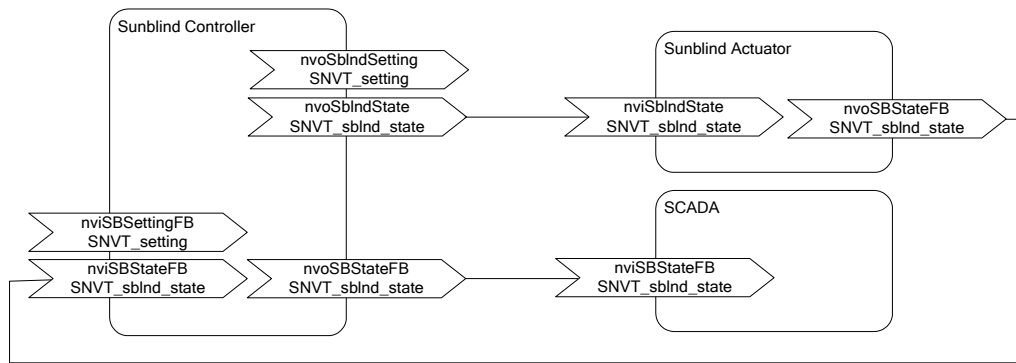
Figure 123: Controlling a Sunblind Actuator via SNVT_sbld_state
