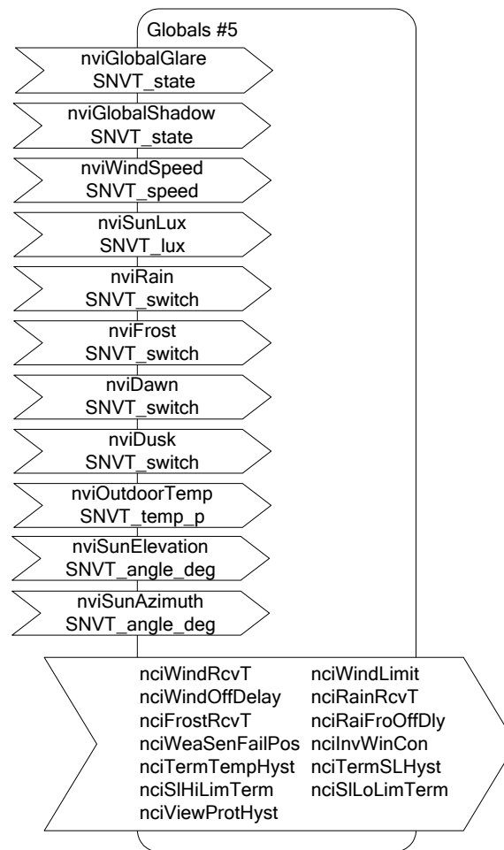
Figure 125: Global Object
