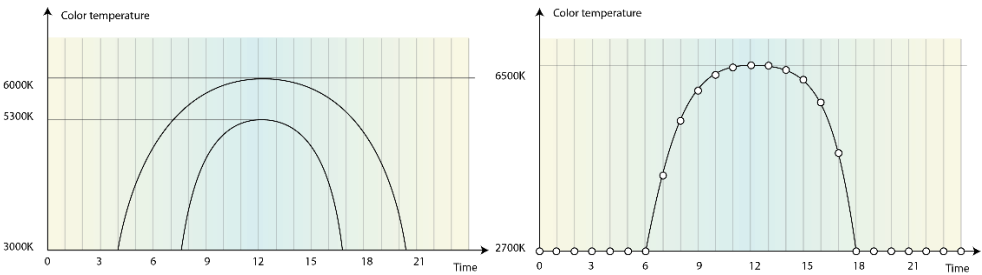
Figure 143: HCL Profile “elevation” based with different Tc max values for summer and winter (left) and “curve daily” with hourly support values (right)
