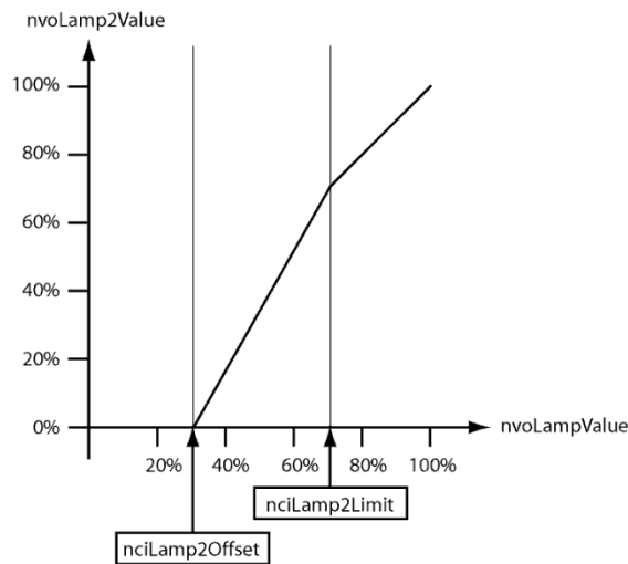
Figure 115: Secondary Light Band
