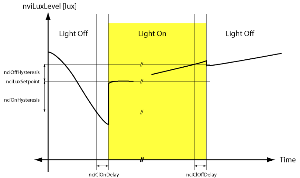
Figure 116: Constant Light Controller Timing
