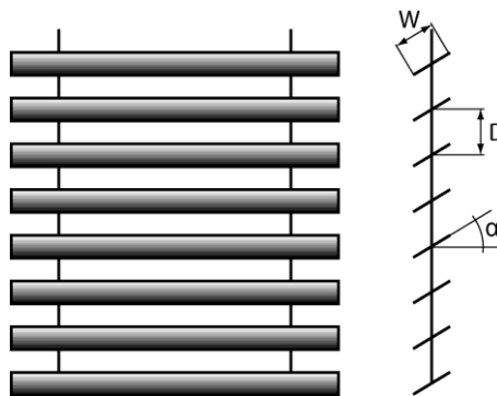
Figure 145: Sunblind Geometry
