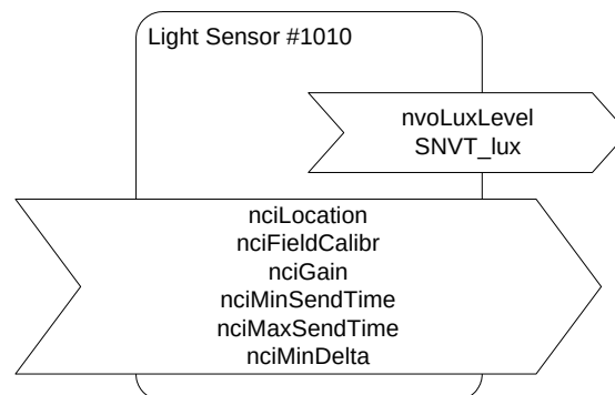
Figure 109: Light Sensor Object
