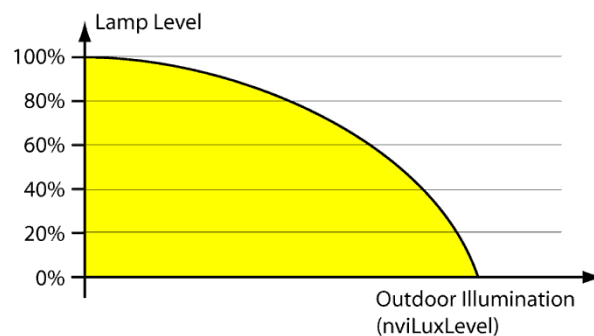
Figure 114: Control Mode
