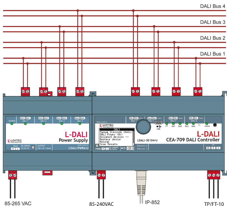
Figure 65: Basic Hardware Installation with external DALI bus power.
