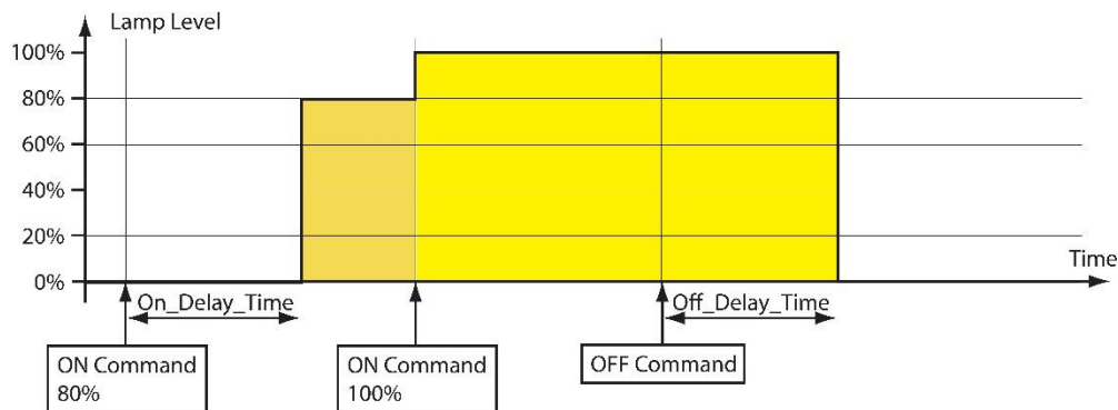
Figure 131: Timing Parameters.
