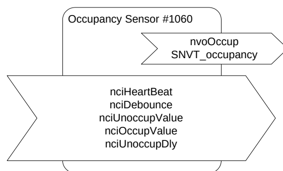
Figure 110: Occupancy Sensor Object.
