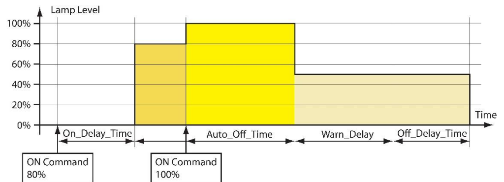
Figure 133: Timing Parameters (restart enabled).
