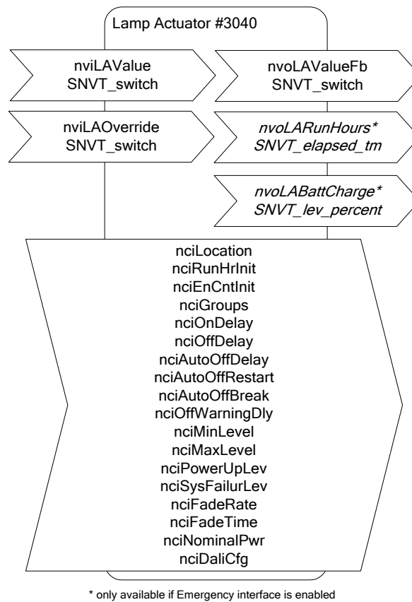
Figure 101: Lamp Actuator Object
