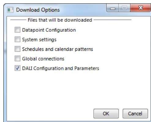
Figure 82: LINX Configurator software, Download DALI Configuration and Parameters.
