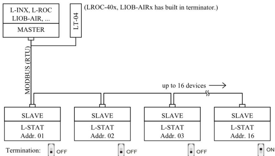
Figure 7: Modbus Network
